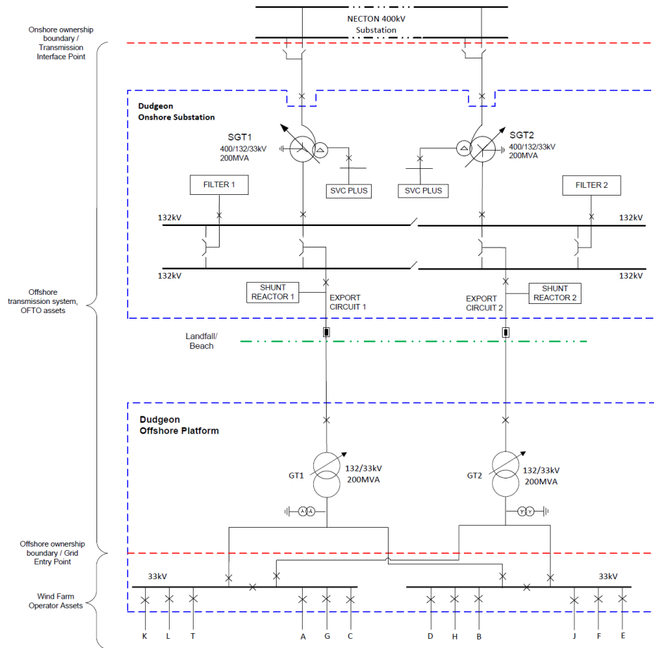
Dudgeon Offshore Wind Farm Simplified single line diagram offshore transmission system
