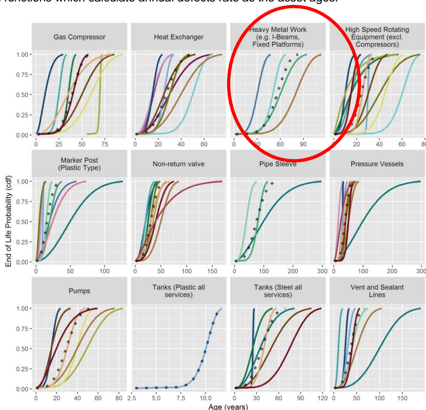
Figure B1 Elicited deterioration curves for Repairable Mechanical assets in the Sites model
