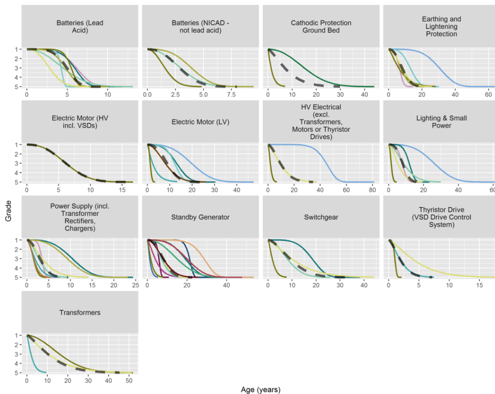
Figure D1 Examples of AH versus Effective Age elicitation curves
