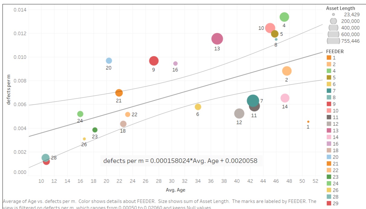
Figure 5 Predicted numbers of new corrosion defects per year based on pipeline age
