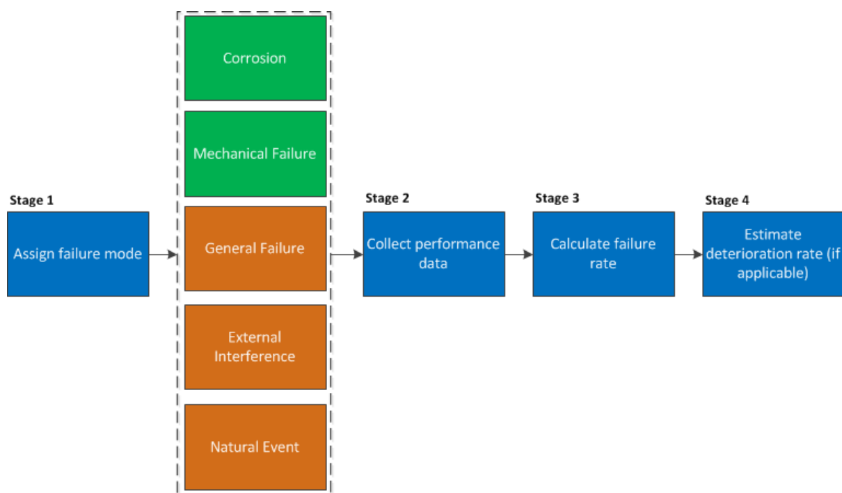
Figure 3 Overview of Pipelines defect/failure rate modelling approach
