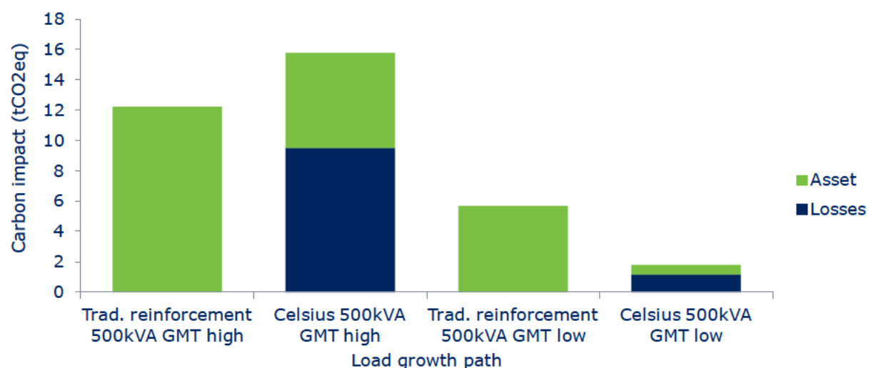
Figure 3.8: Carbon impact of traditional reinforcement and Celsius
