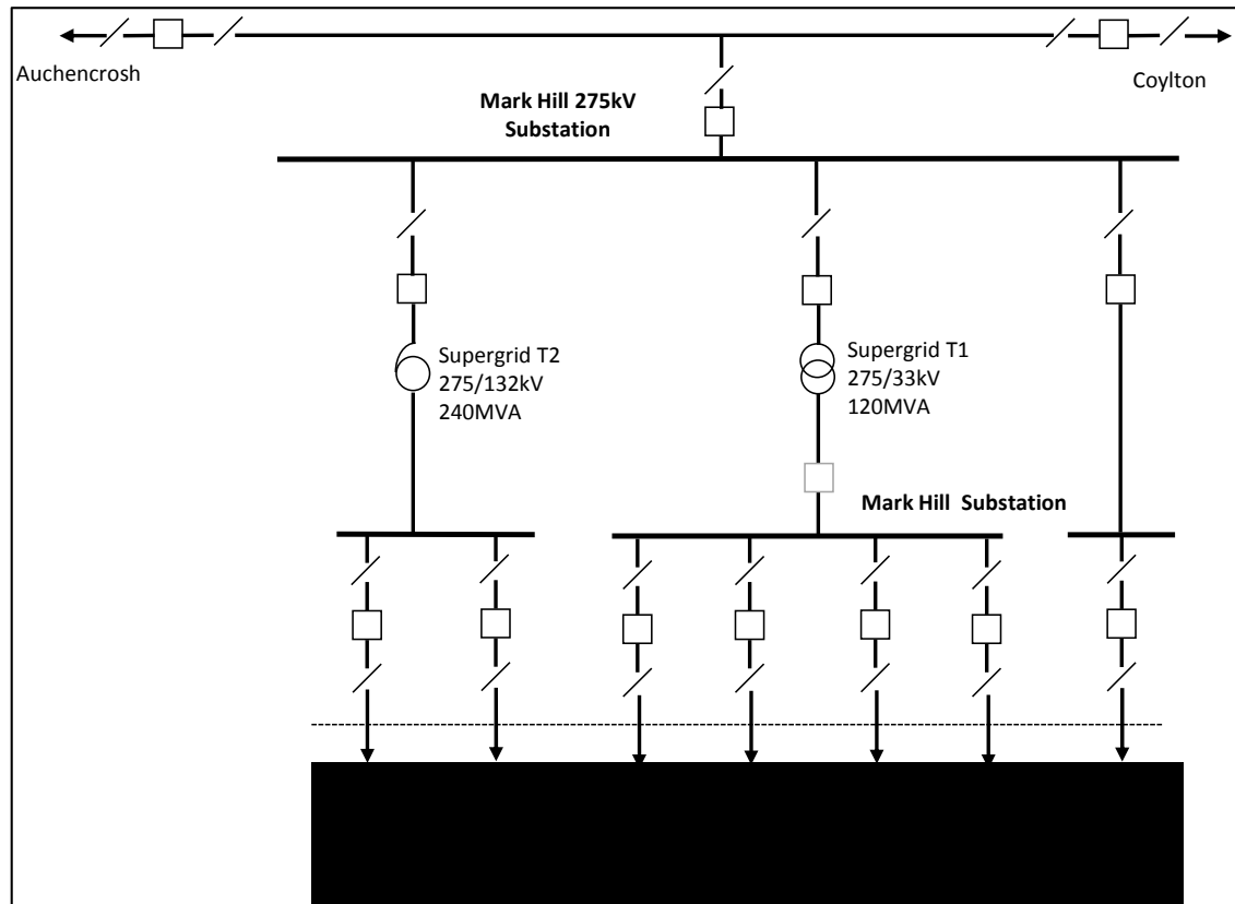
Figure 7. YY Route Schematic and connected and contracted generation connections
