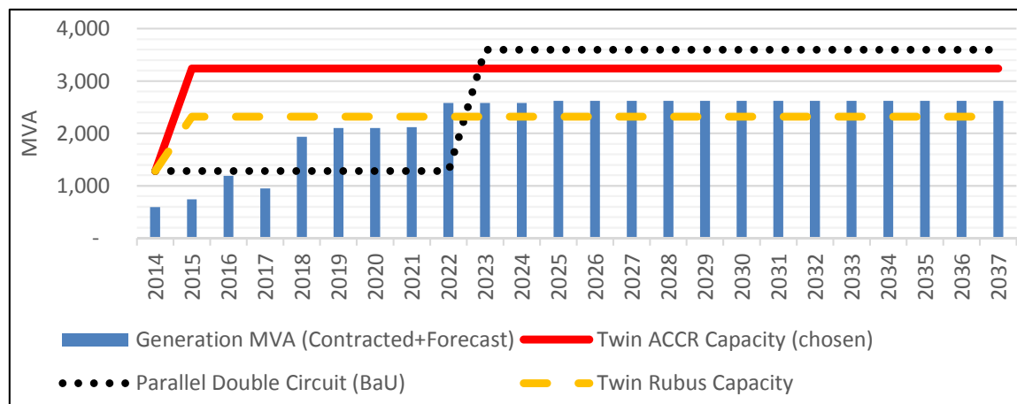
Figure 12. CBA-2 capacity outputs, chosen ACCR Drake versus new parallel circuit and twin Rubus option anticipated within the SWS Project set out in the Business Plan.
