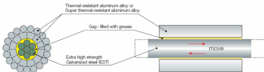
Figure 5. Cross-section of gap-type Aluminium Conductor Steel Reinforced (GTACSR)
