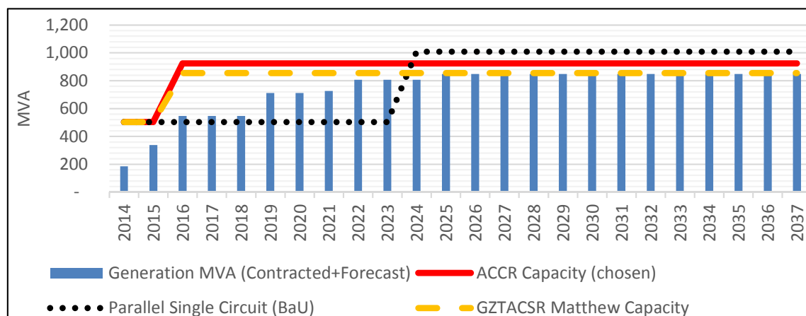
Figure 11. CBA-1 capacity outputs, chosen ACCR Curlew versus baseline new build
