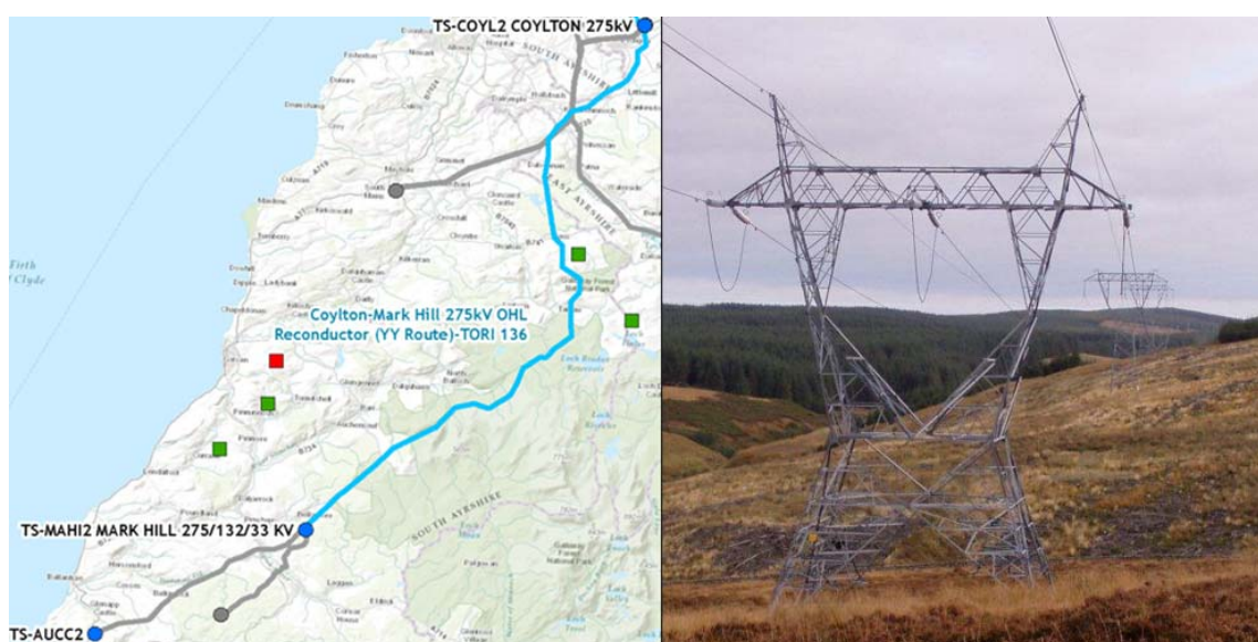
Figure 8. GIS map of the route and photograph of a LR tower, aka. "Cats head"
