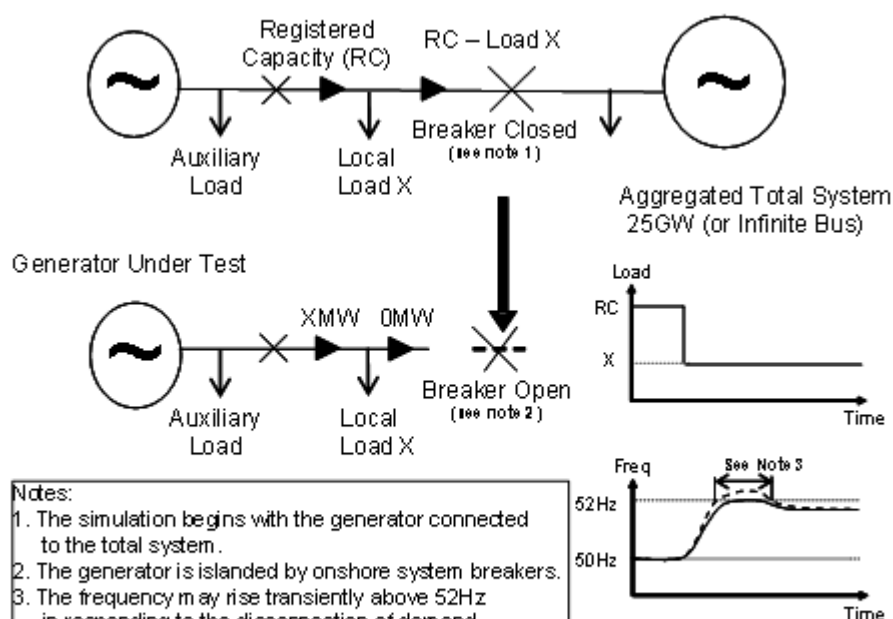
Generator Under Test
