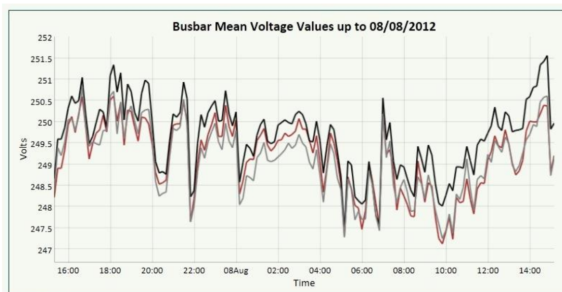
Fig 13 – Typical voltage profile – Ritchie Gdns (WPD) –Gridkey
