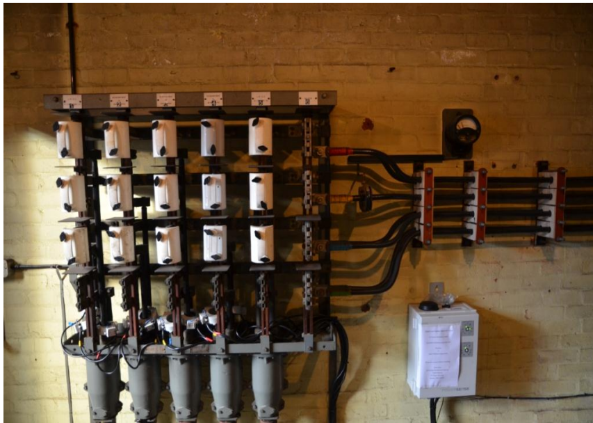
Figure 15: Installation of CTs and DISCOS metrology unit from PowerSense. (UKPN)
