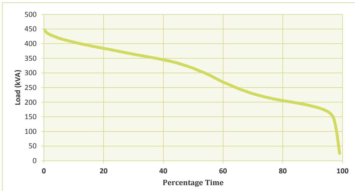
Fig 15 – Load Duration Curve –Dean Street (UKPN) – GMC-iProslys / Nortech
