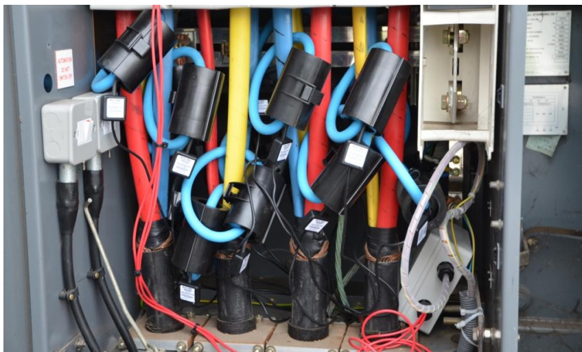
Figure 9: Blue Rogowski coils by Current Grid in congested LV cabinet. (WPD)
