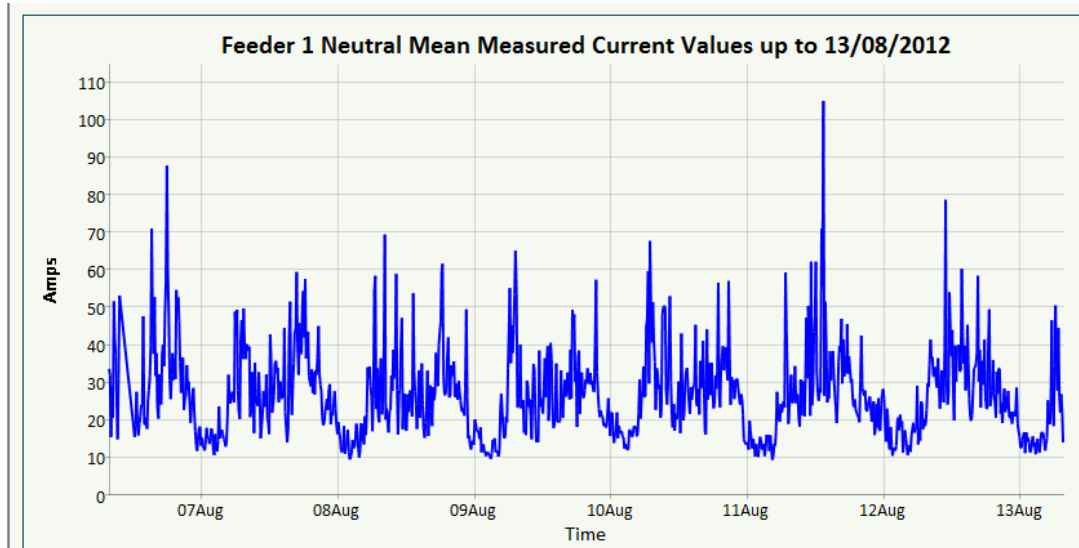
Fig 14 – Neutral Current from network imbalance – Ritchie Gdns (WPD) -Gridkey
