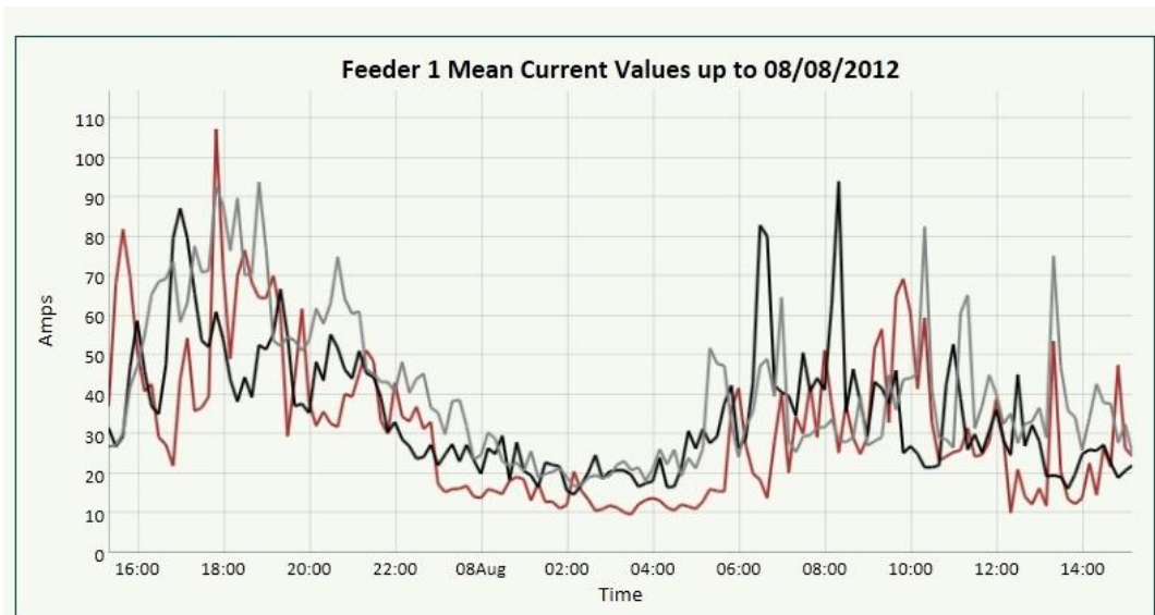
Fig 12 – Typical Load Profile – Ritchie Gdns (WPD) -Gridkey
