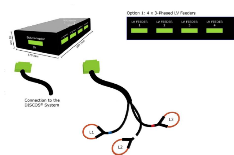
Figure 16: PowerSense LV satellite box and Rogowski coils
