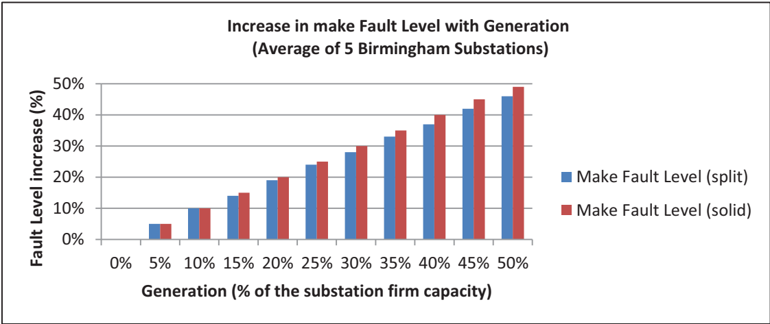
a) Average increase in make Fault Level with generation
