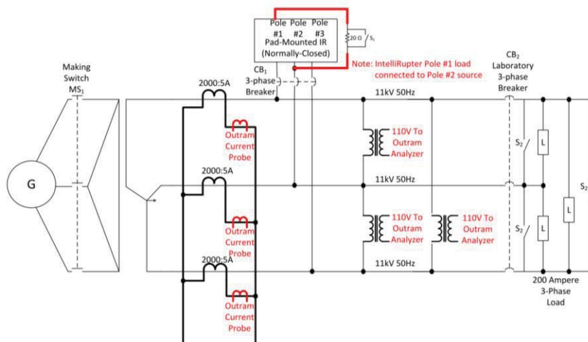
Figure 1. Laboratory Test Set-Up
