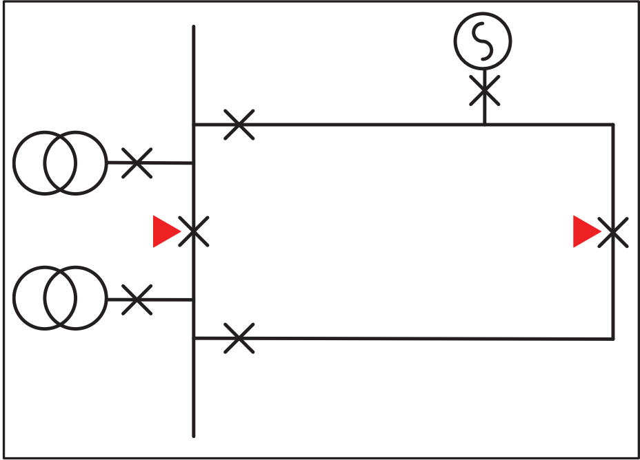
a) Split configuration (open)
