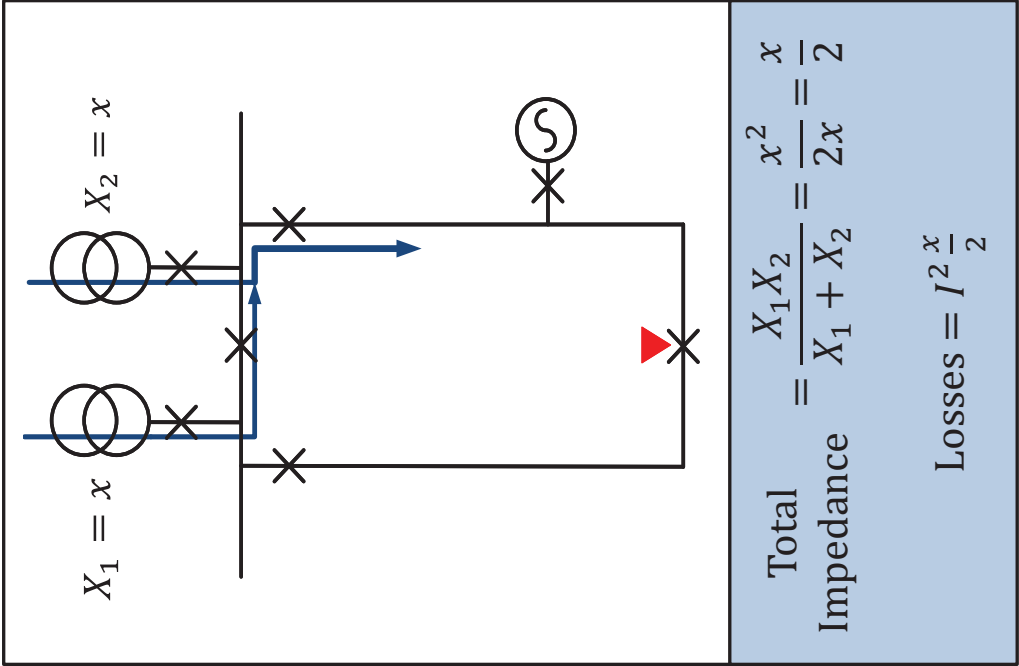
b) Losses for solid configuration
