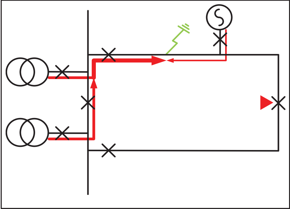
b) Fault in-feed for solid configuration
