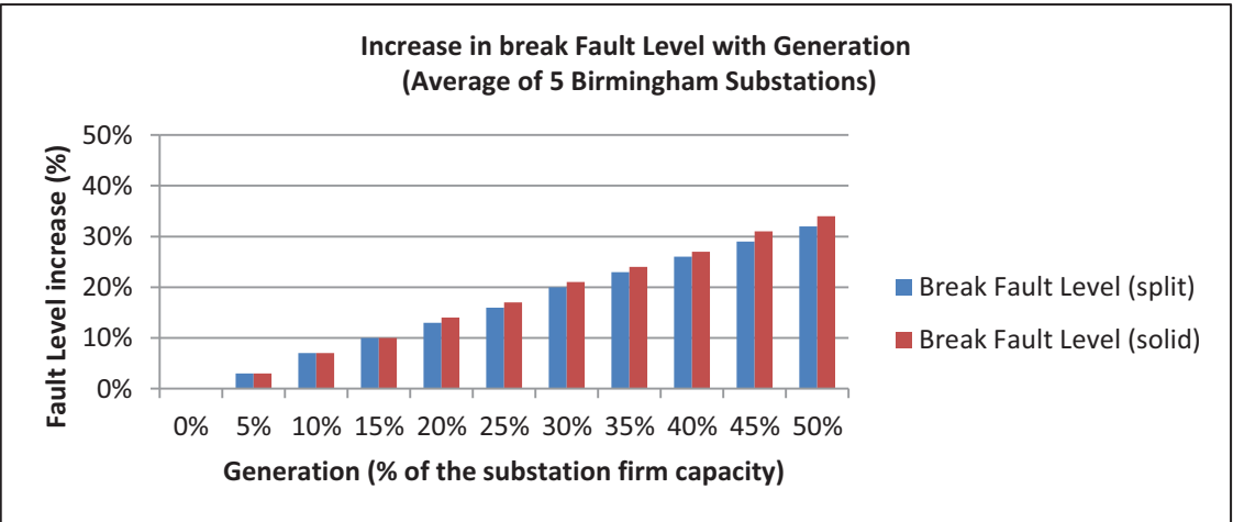
b) Average increase in break Fault Level with generation
