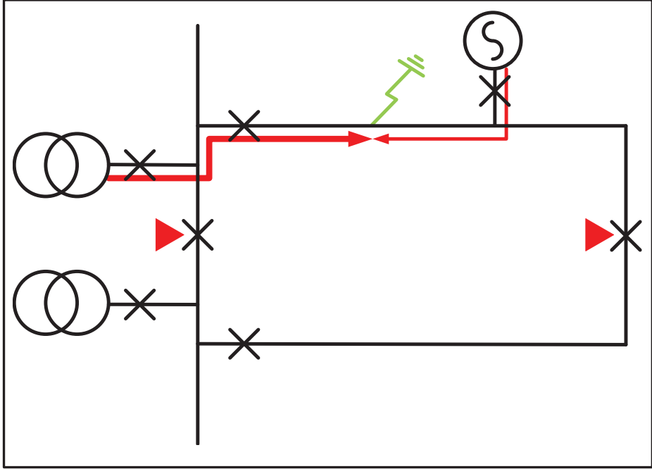
a) Fault in-feed for split configuration
