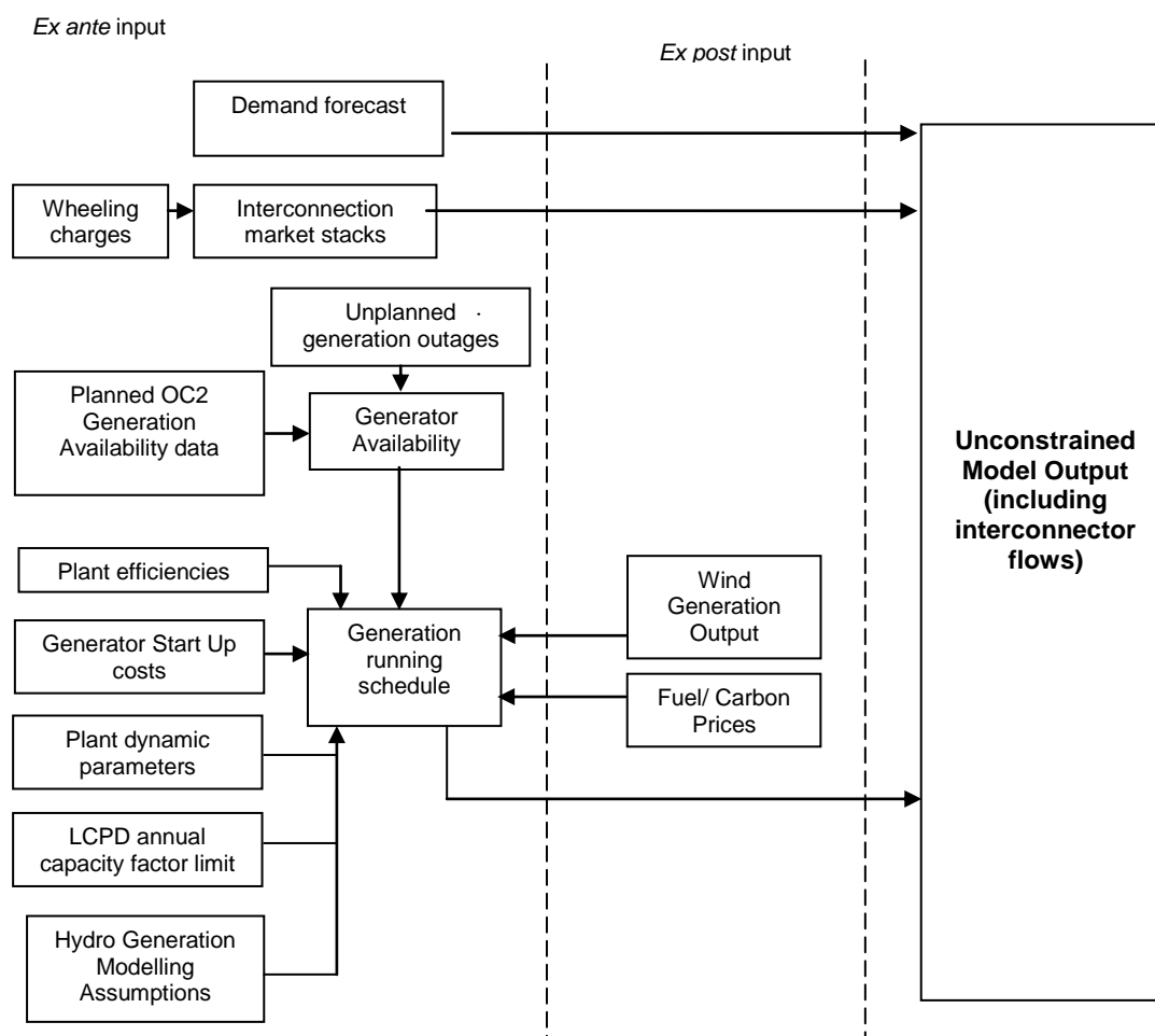
Figure 4: Unconstrained Output Model
