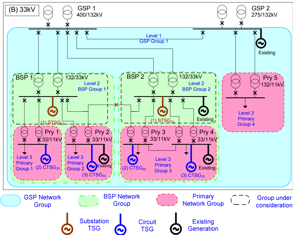
Figure 14 - Example of Test Size Generators application and testing at the 33kV network level
