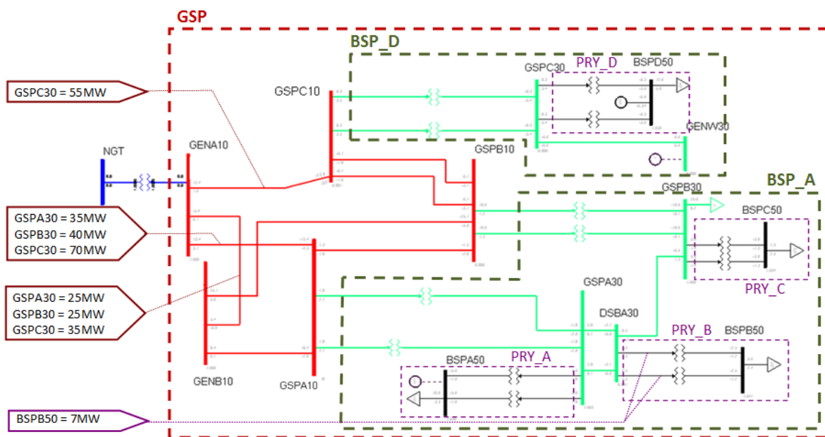
Figure 17 - Example of generation charging by Network Groups
