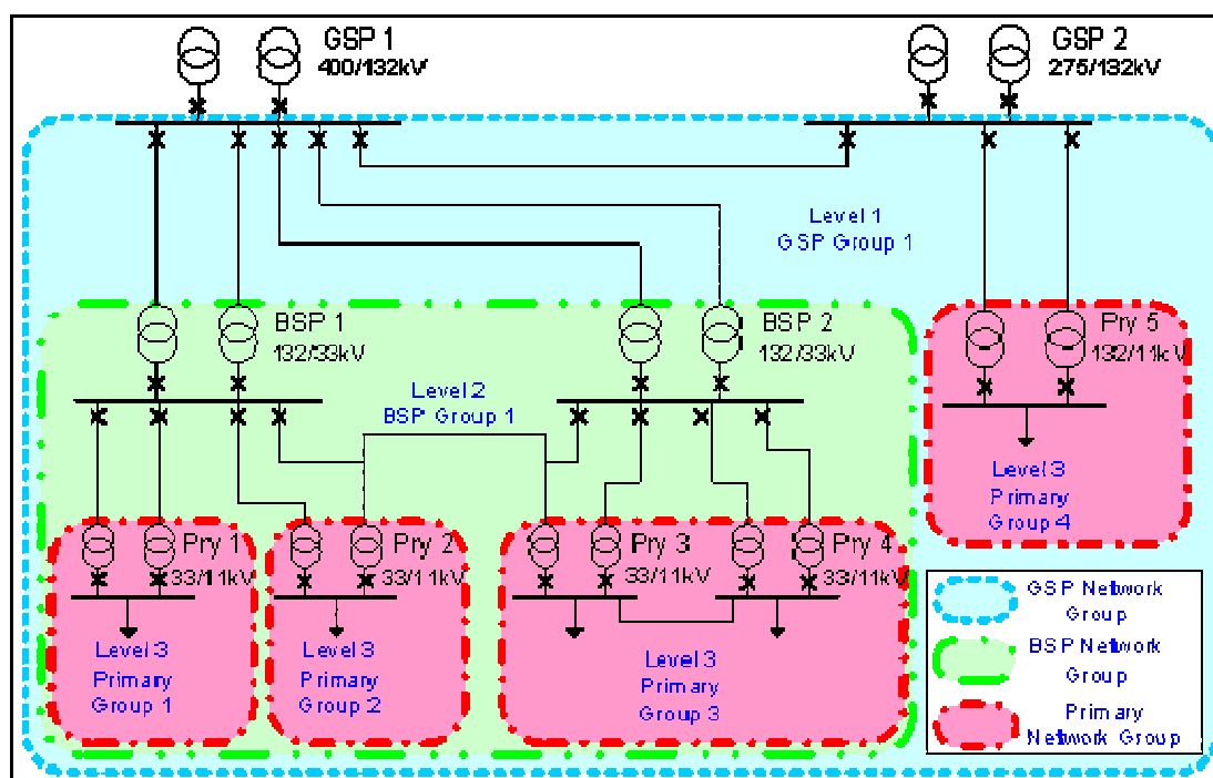
Figure 9 - Example network showing three levels of Network Groups.
