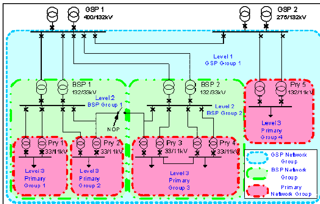
Figure 10 - Example network similar to Figure 6 showing that the addition of the Normally Open Point (NOP) has created two level 2 BSP Network Groups.
