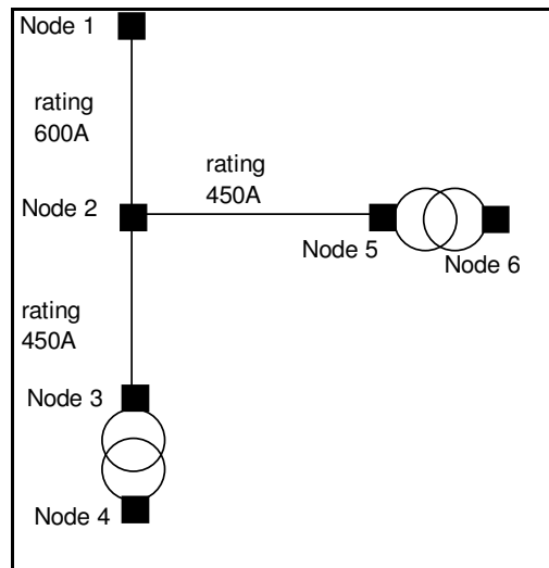
Figure 4 - The resultant nodal model representative of the example network in Figure 1.
