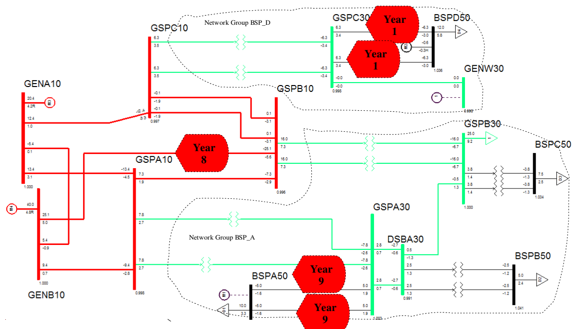
Figure 16 - Example of charging by Network Groups
