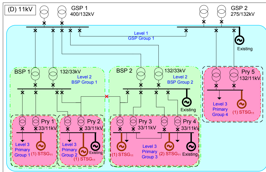
Figure 15 - Example of Test Size Generators application and testing at the 11kV network level
