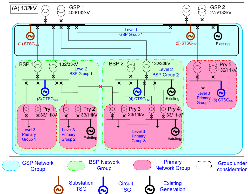
Figure 13 - Example of Test Size Generators application and testing at the 132kV network level
