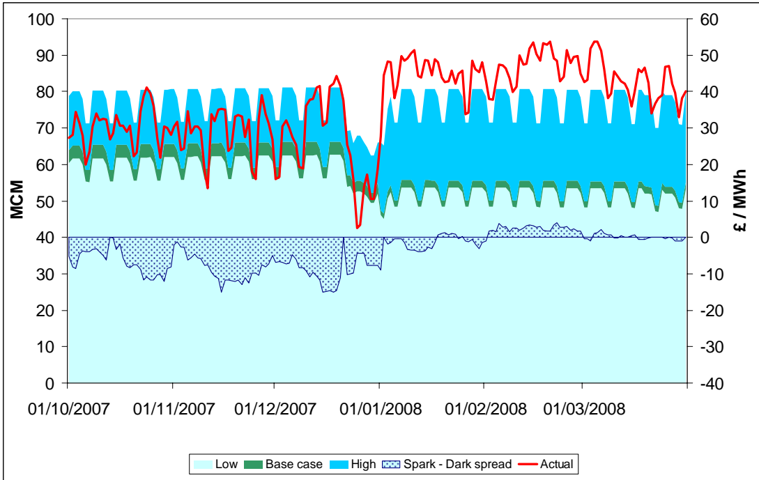
Figure A.12 – 2007/8 Actual Power Station Demand
