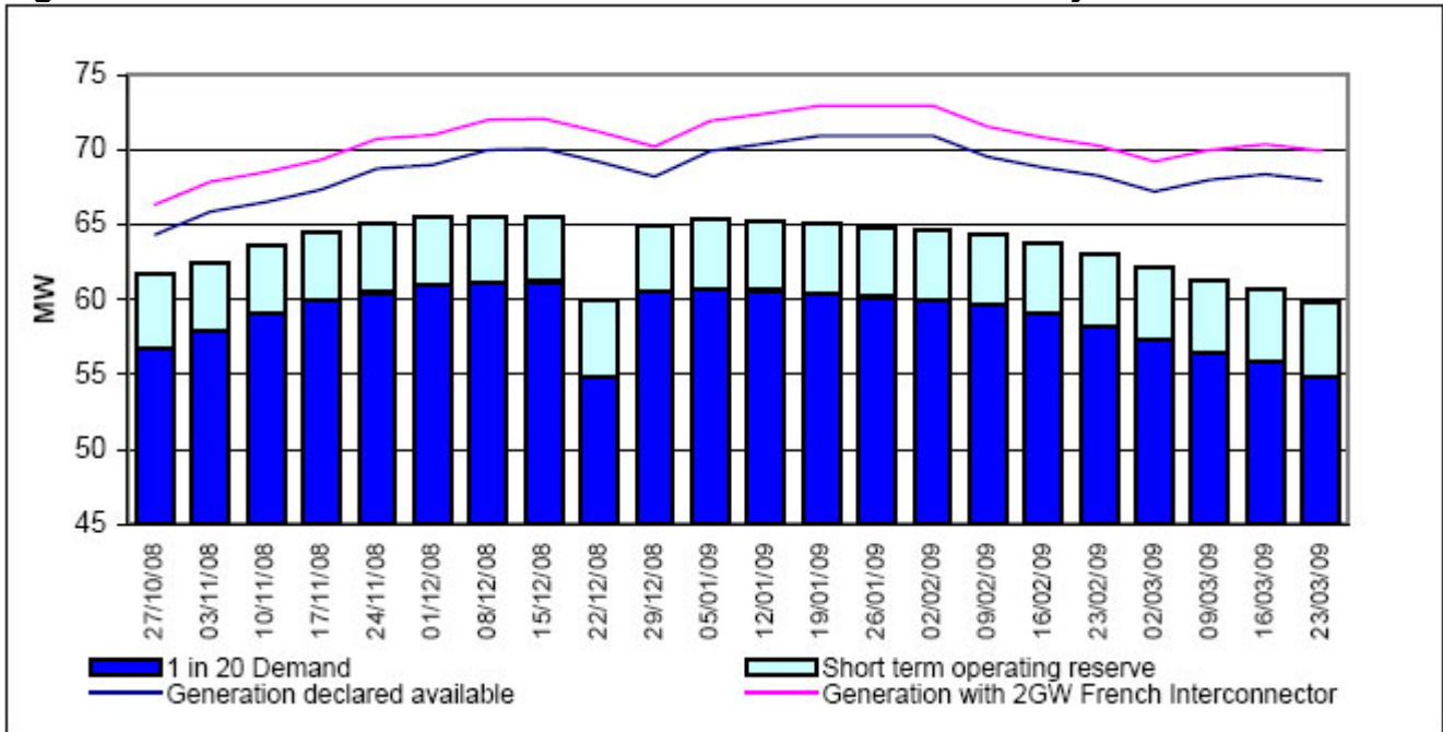
Figure B.19 - 1 in 20 Demand and Notified Generation Availability
