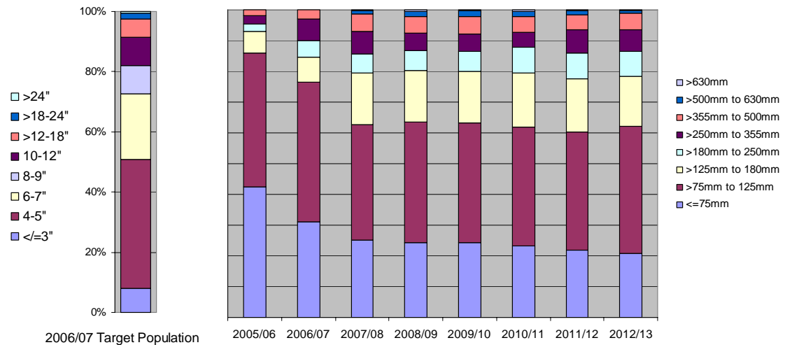
Proposed Diameter Mix for Replacement
