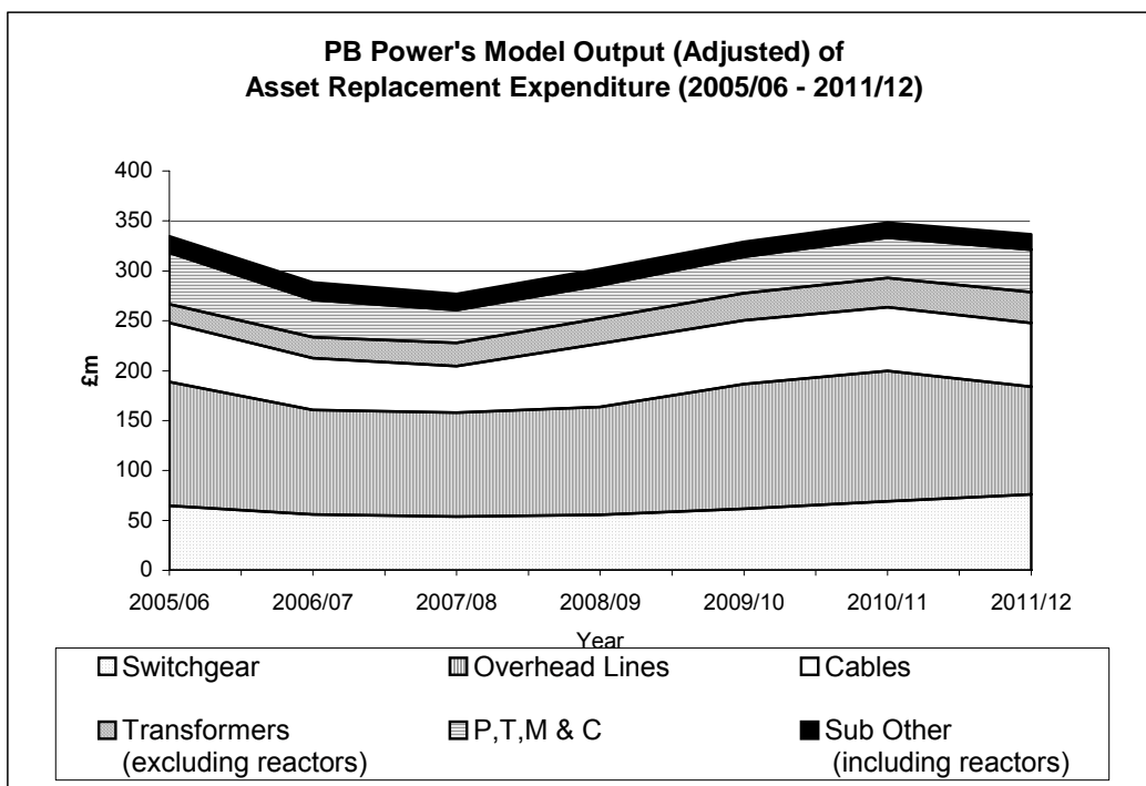
Figure 4.6 – PB Power’s model output of asset replacement expenditure
