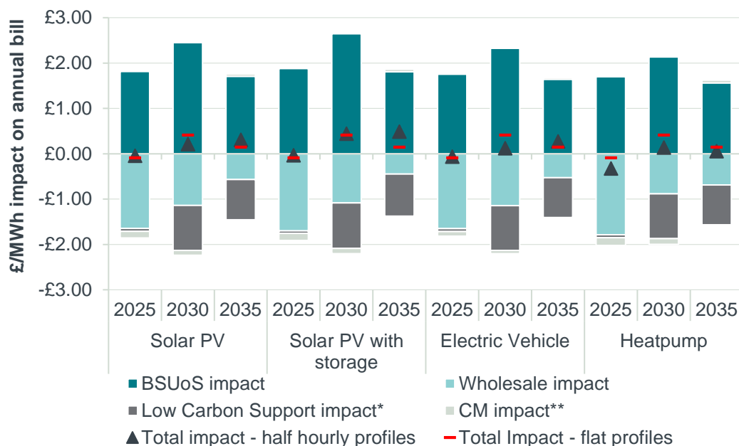
Figure 44 Steady Progression – Annual £/MWh impact – Domestic with low carbon technologies
