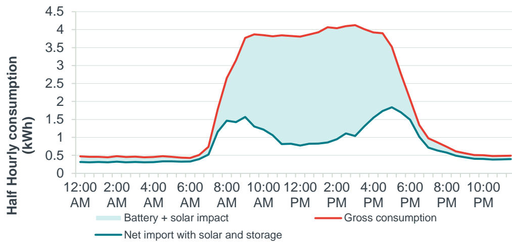
Figure 41 High usage commercial customer annual half hourly net consumption profile with storage unit – Autumn weekday
