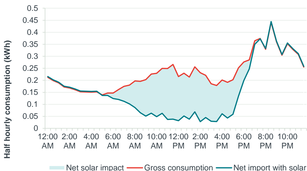
Figure 35 Impact of solar PV installation on consumption of medium domestic consumer (without storage) – Average spring weekday consumption
