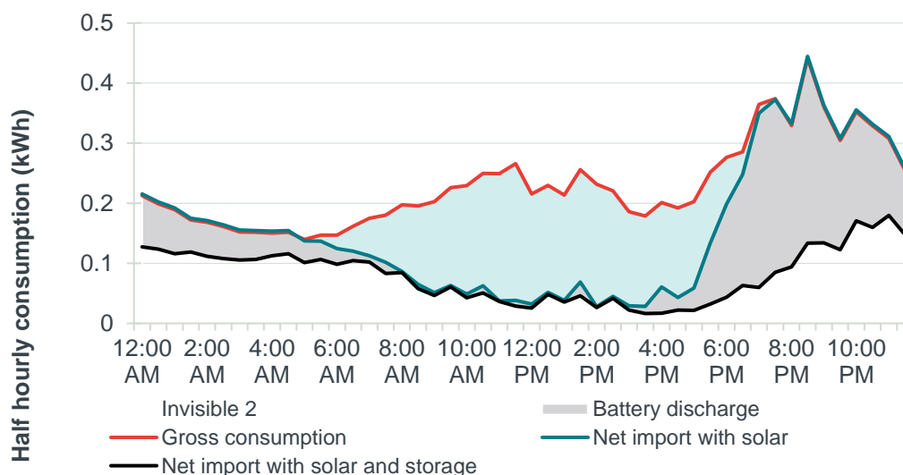
Figure 36 Impact of solar PV installation and storage on consumption of medium domestic consumer – Average spring weekday consumption
