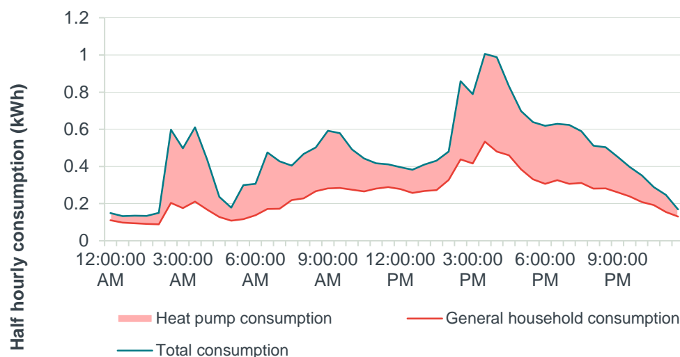
Figure 38: Average consumption of a domestic customer with a heat pump
