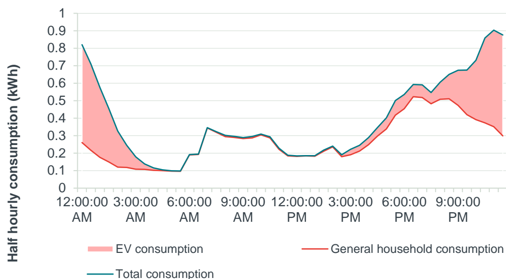
Figure 37: Average consumption of an electric vehicle customer
