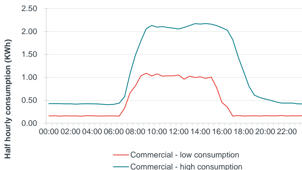
Figure 40 Average annual half-hourly consumption profile for representative low and high commercial users
