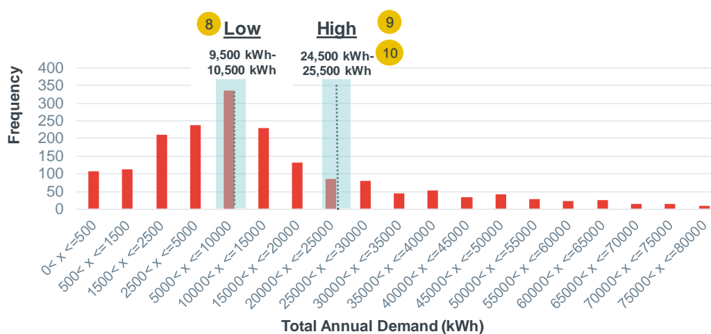
Figure 39: Distribution of annual demand for commercial customers in CLNR dataset
