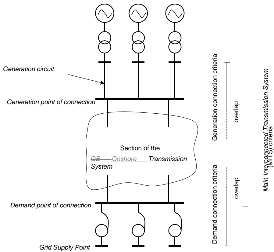
Figure 1.1 The GB onshore transmission system with a directly connected power station
